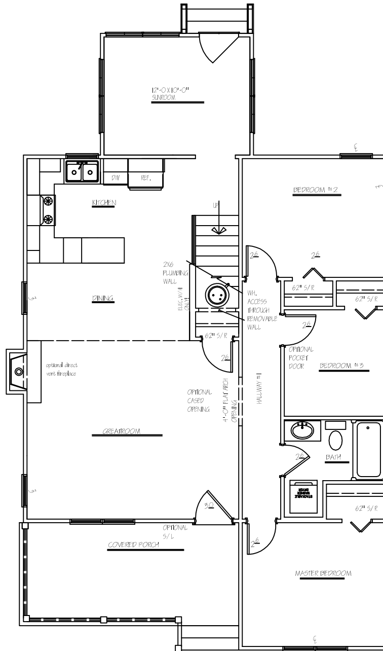
1ST FLOOR PLAN SHOWN WITH OPTIONAL SUNROOM
